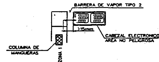
DETALLE "E"
